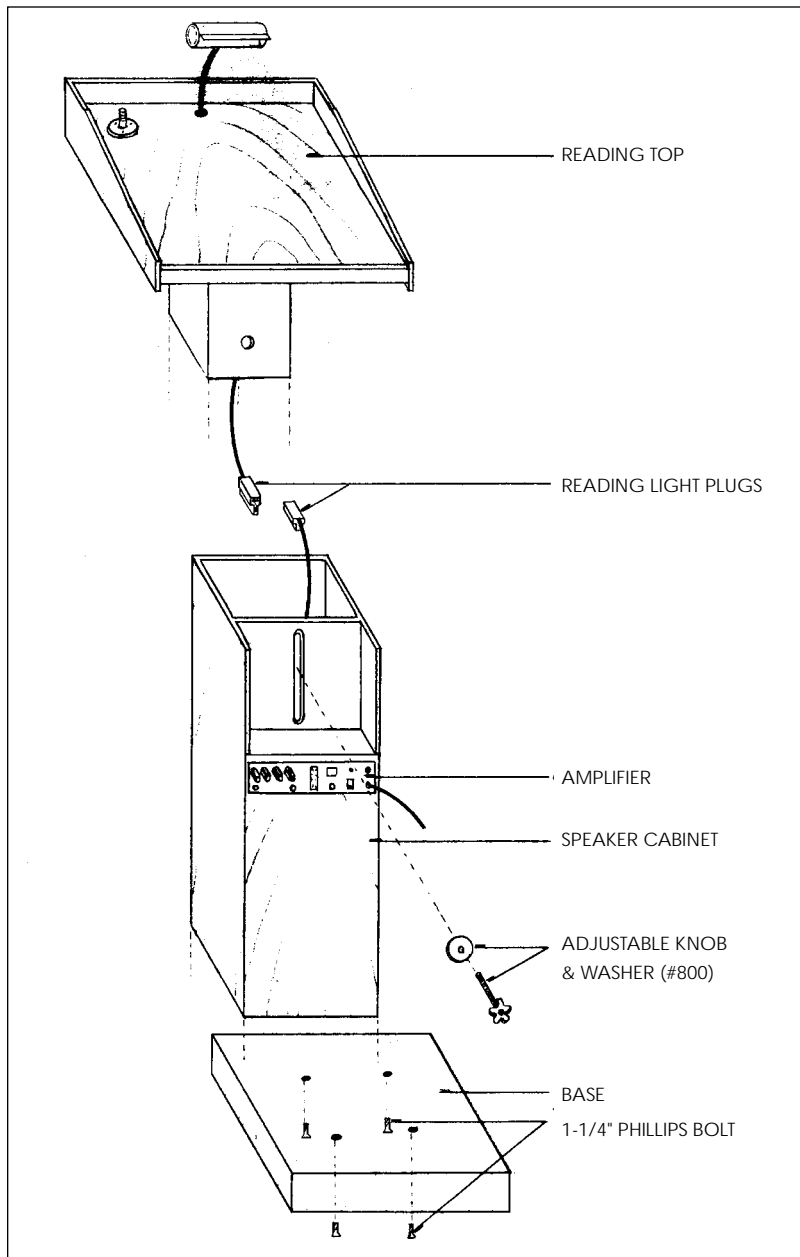
ASSEMBLY DIAGRAM FOR MODEL 800
